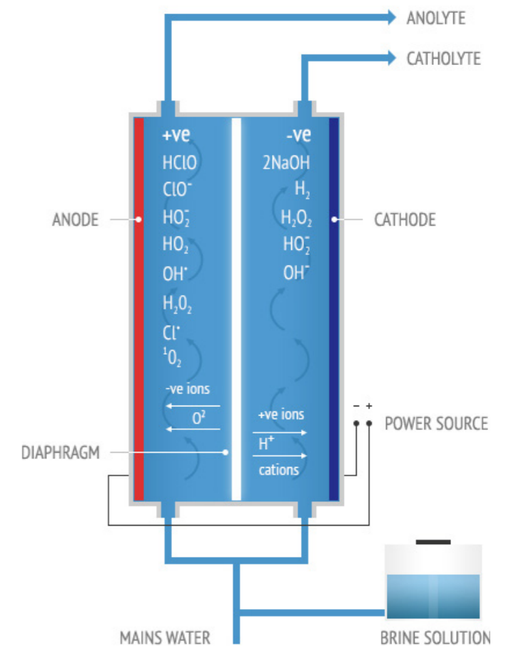
Drawing of Enviolyte operational principle
