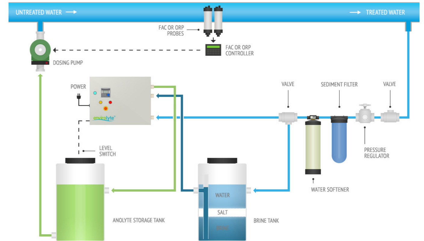
Typical layout of Enviolyte water disinfection system
